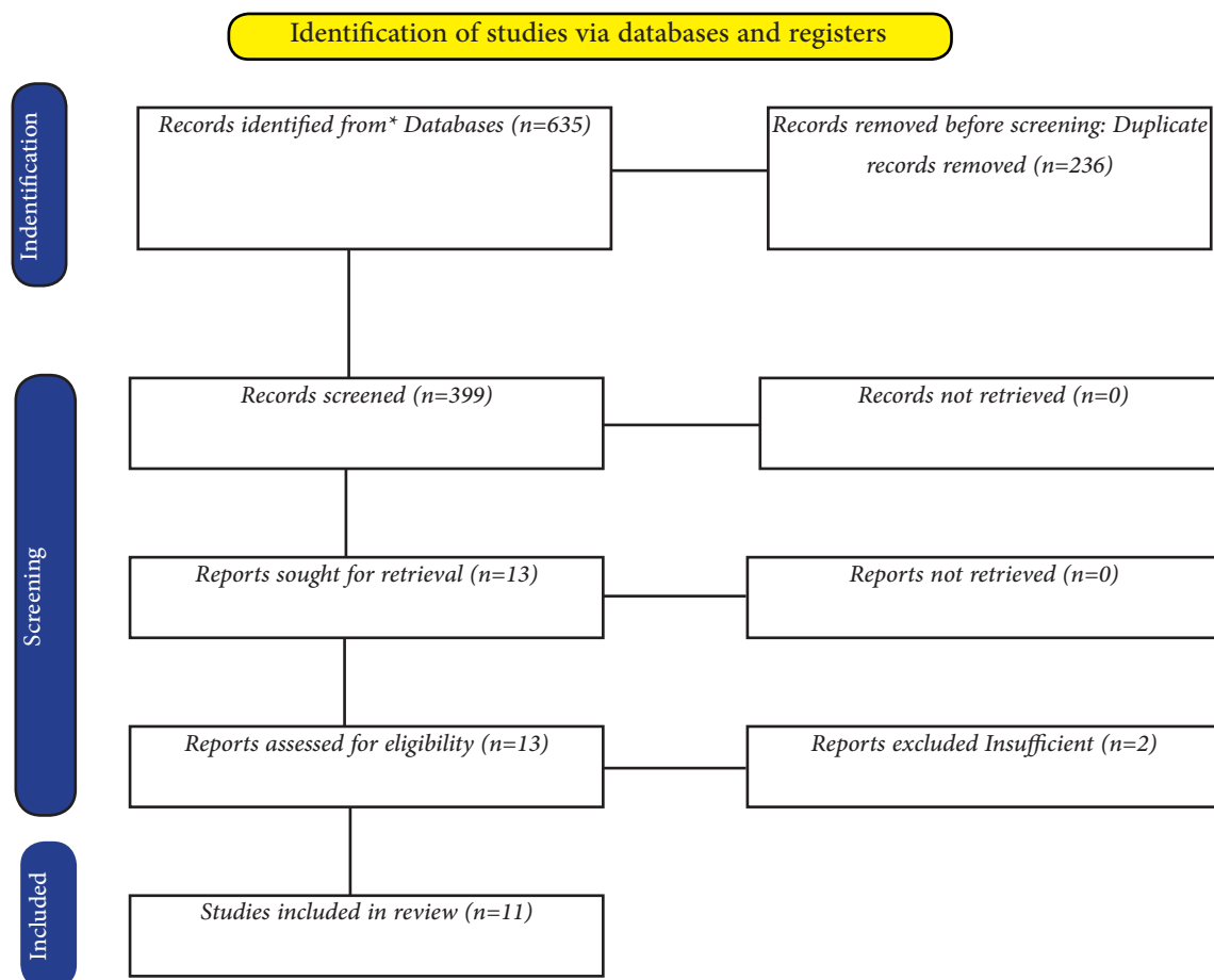
Figure 1. PRISMA flowchart.
